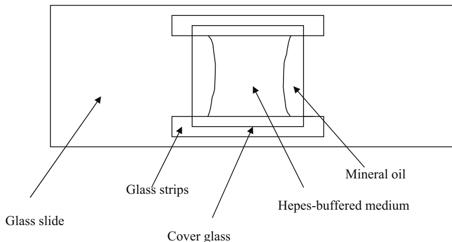
Fig. 8.2. Manipulation chamber
