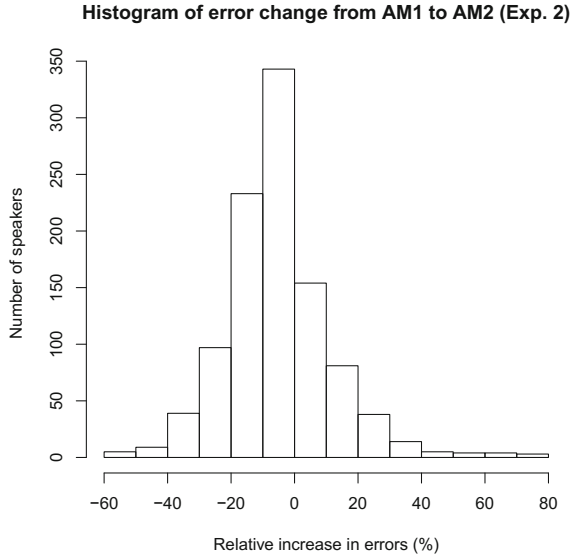
Fig. 3. Relative WER change by speaker, AM1 to AM2 (Experiment 2).
