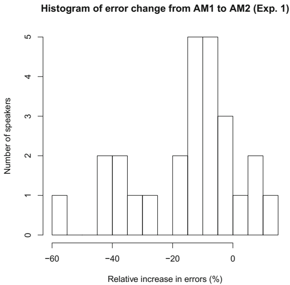
Fig. 2. Relative WER change by speaker, AM1 to AM2 (Experiment 2)
