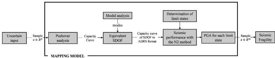
Fig. 3. Scheme of the adopted methodology of vulnerability assessment including material uncertainty
