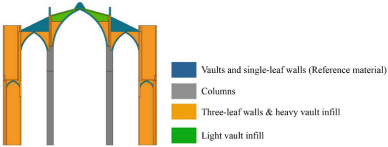
Fig. 1. Categorization of the structural members in the representative bay of the church of Santa Maria del Mar.
