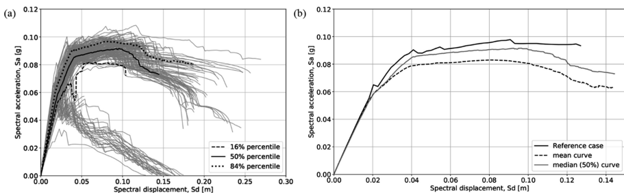
Fig. 4. (a) The obtained capacity curves of the 200 performed analyses, (b) Mean, median and reference capacity curves
