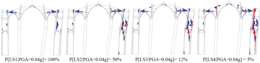
Fig. 9. Correspondence between limit states and cracking for an analysed case of a local collapse not involving the left buttress
