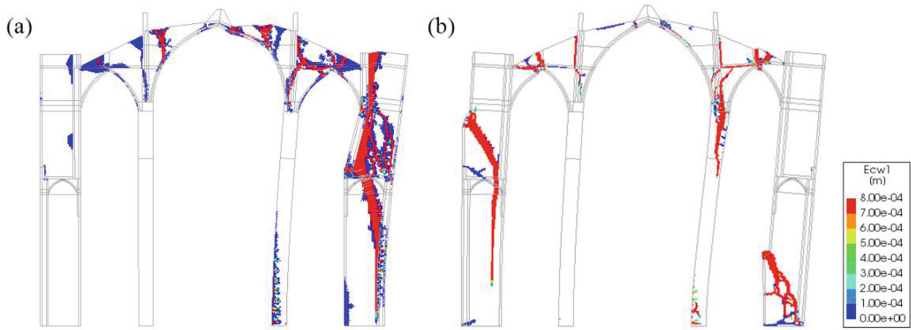
Fig. 5. Crack widths at the end of the analysis in: (a) case with a collapse mechanism characterized by the shear failure of the right buttress, (b) case with a global collapse mechanism involving the main and lateral vaults and the two lateral buttresses of the structure.
