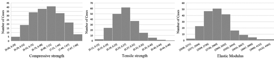
Fig. 2. Distribution of compressive strength, tensile strength and elastic modulus for the reference material.
