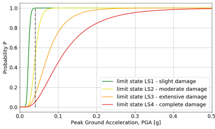
Fig. 6. Fragility curves for each limit state in terms of PGA
