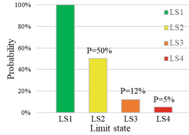
Fig. 7. Probability of occurrence of each limit state for PGA = 0.04 g
