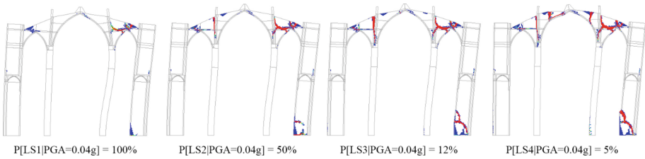
Fig. 8. Correspondence between limit states and cracking for an analysed case of a global collapse mechanism
