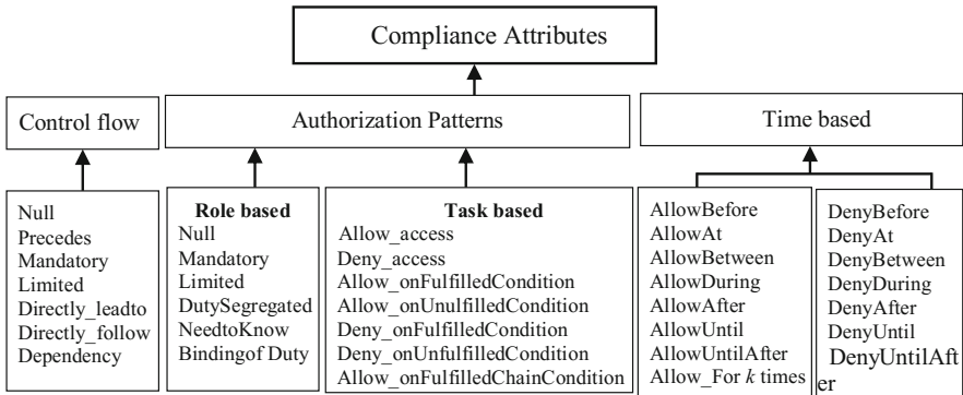
Fig. 2. Compliancy attributes meta-model
