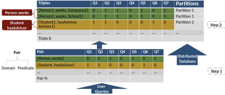
Fig. 1. Dataset construction.
