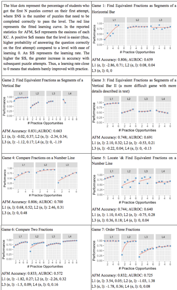
Fig. 1. Learning curve plots and AFM statistics.
