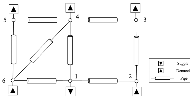
Fig. 3. Topology of the ring pipeline network in case 2
