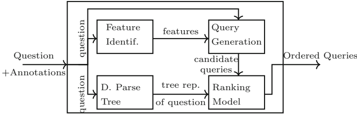
Fig. 2. The architecture of SQG
