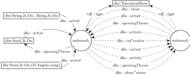
Fig. 3. The captured subgraph for the given question, annotated with candidate entities and relations; solid lines are the one that are in one hop distance; dashed line means more than one hop distance; circles represent unbound nodes, rectangles are the linked entities and edges are the relations in the KG.
