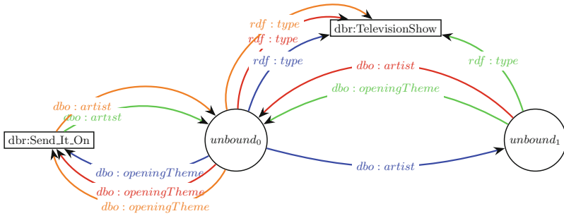
Fig. 4. Four candidate walks are found which are shown in different colors (Color figure online)
