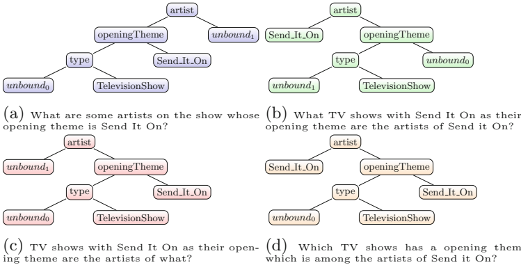
Fig. 6. Tree representation of the candidate walks along with their NL meaning
