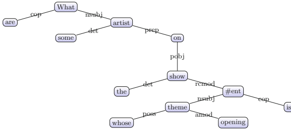
Fig. 5. Dependency parse tree of the running example
