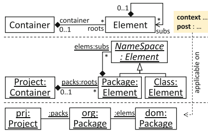
Fig. 9. Reuse by multilevel modeling
