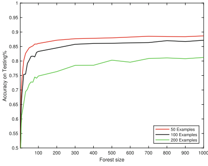
(a) Mean testing accuracy across all datasets for PLP-forests applying Top-2 Clusters, where every member tree is trained using random samples of sizes 50, 100 and 200.
