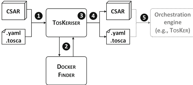
Fig. 6. How TOSKERISER works.
