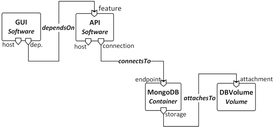
Fig. 4. A specification of our running example in TOSCA (where nodes are typed with tosker.nodes.Container , tosker.nodes.Volume , or tosker.nodes.Software , while relationships are typed with TOSCA normative types [18]).
