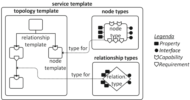
Fig. 2. The TOSCA metamodel [18].
