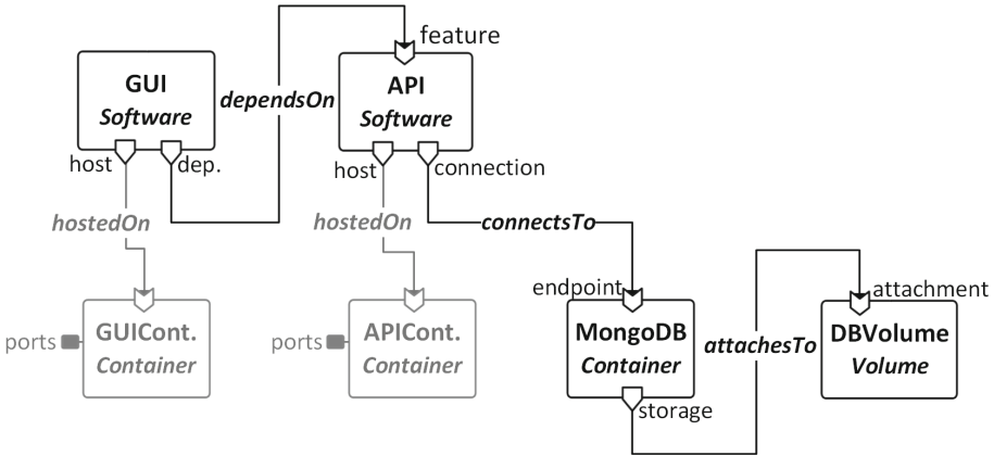
Fig. 7. Application topology obtained by completing the partial topology of the application Thinking (Fig. 4). Lighter nodes and relationships are those automatically included by TOSKERISER.
