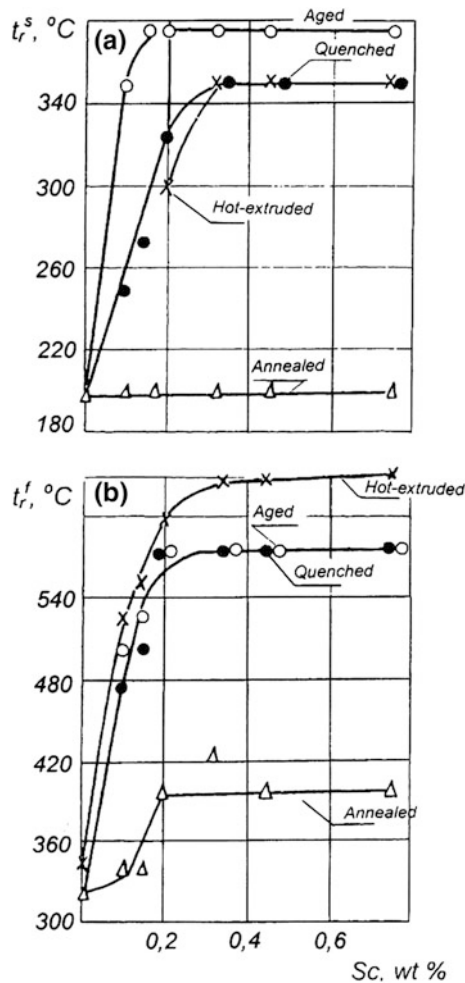
Fig. 8 Effect of Sc additions on the recrystallization temperature of aluminum: a recrystallization onset and b recrystallization completion. After [18]
