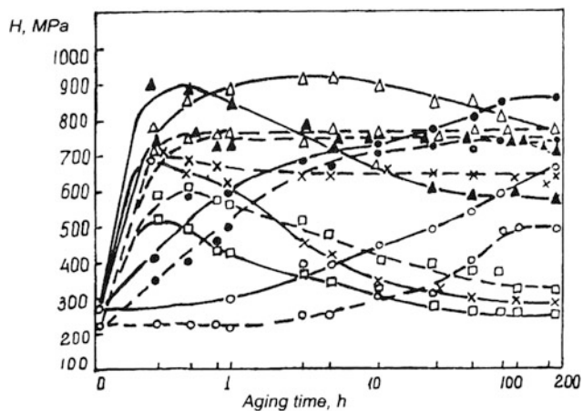
Fig. 6 Aging curves for Al-0.3% Sc (solid lines) and Al-0.3% Sc-0.17% Zr (dashed lines) at 200 °C (O); 300 °C (●); 300 °C (Δ); 350 °C (▲); 400 °C (×); and 450 °C (□). After [9]
