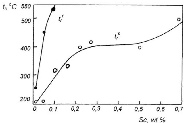
Fig. 9 Effect of Sc concentration of the recrystallization temperatures in an Al-6.5% Mg alloy. After [9]
