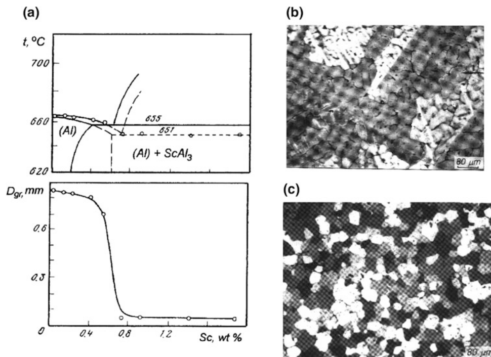
Fig. 11 Grain refining upon solidification of Al–Sc alloys: a correlation of the grain refining with the composition; b an Al–Mg alloy and c an Al–Mg–Sc–Zr alloy
