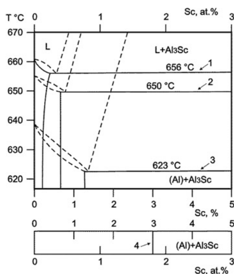
Fig. 1 Metastable phase diagrams of the Al–Sc system as 5 K/s (1); 10^2 K/s (2); 10^3 K/s (3) and 10^5 K/s (4). After [9]
