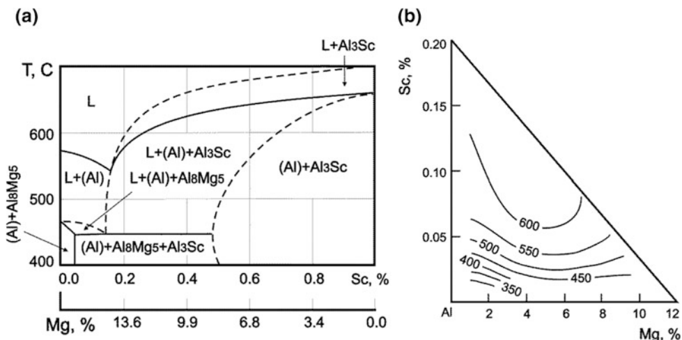
Fig. 3 a A polythermal section from Al–17% Mg to Al–1% Sc of the Al–Mg–Sc phase diagram and b solid solubility of Mg and Sc in (Al). After [9]
