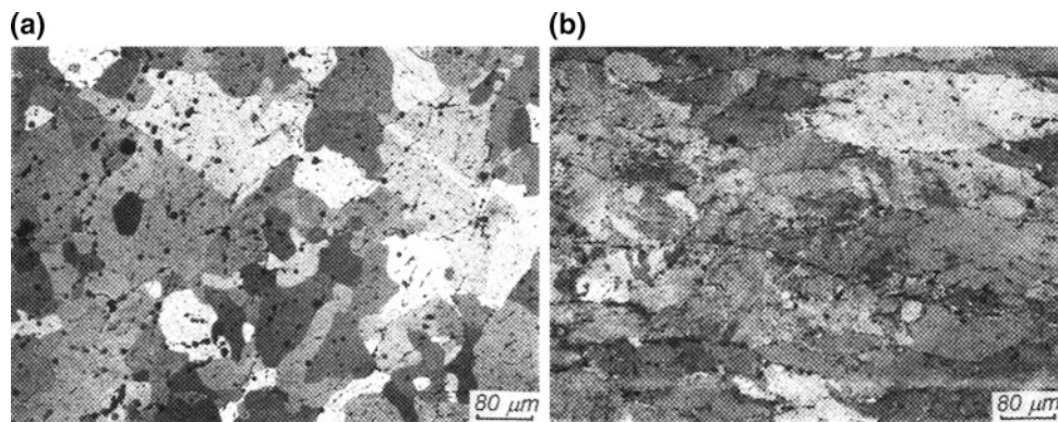
Fig. 10 Grain structure of an AA6XXX alloy after homogenization at 480 °C, hot rolling at 400 °C and quenching from 500 °C: a an alloy without Sc and Zr and b an alloy with Sc and Zr. After [32]
