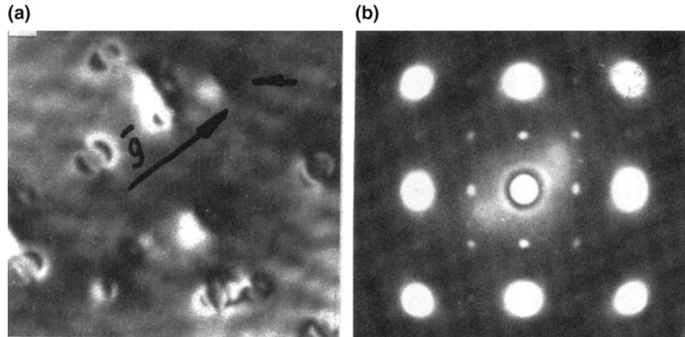
Fig. 4 Precipitation of coherent \text{Al}_3\text{Sc} particles in an Al-0.6% Sc alloy at 350 °C, 100 h: a microstructure showing particles 13 nm in diameter and b (100) electron diffraction pattern showing superstructure reflections. After [9]
