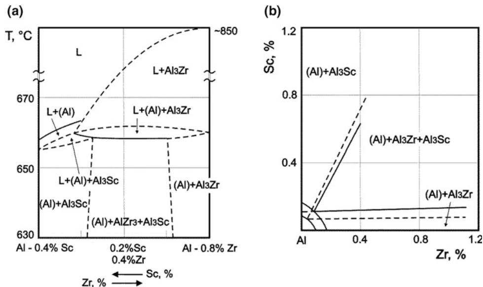
Fig. 2 Section of the Al–Sc–Zr phase diagram: a polythermal section from Al–0.4% Sc to Al–0.8% Zr and b isothermal sections at 550 °C (dashed lines) and 600 °C (solid lines). After [9]
