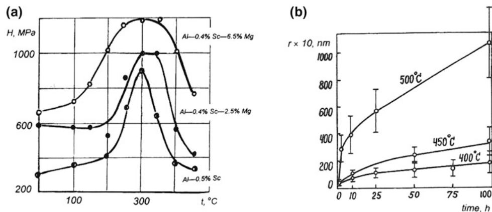
Fig. 5 Effects of precipitation in Al-Mg-Sc alloys: a hardening in binary Al-Sc and ternary Al-Mg-Sc alloys and b evolution of \text{Al}_3\text{Sc} radius during aging of an Al-6.5% Mg-0.4% Sc alloys at different temperatures. After [9]
