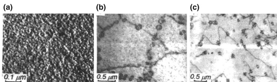
Fig. 7 Precipitation in an Al-0.3% Sc-0.17% Zr alloy: a 350 °C, 200 h; b 400 °C, 200 h; and c 450 °C, 10 h. Larger particles in b are the equilibrium Al_3Sc phase while smaller particles in c are the metastable Al_3Zr phase. After [9]
