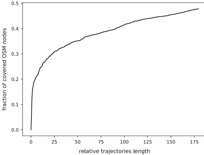
Fig. 3 Fraction of OSM nodes which are covered by at least one trajectory as a function of relative trajectory length defined as the ratio between the total length of all trajectories up to a point in time and total length of the road infrastructure. For close to 100% coverage one would need to have very, very, large trajectory dataset
