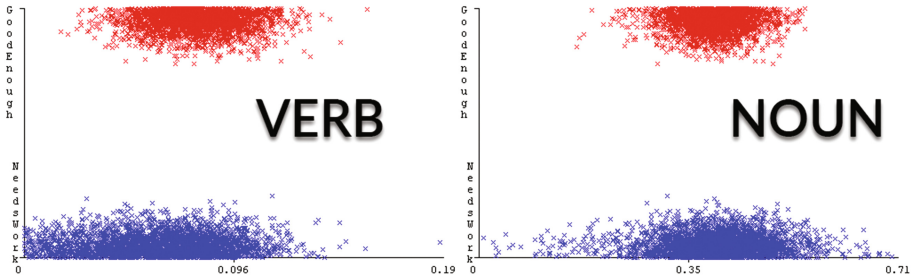
Fig. 2. Distribution of normalized features (by the number of words) in quality classes. Source: own calculations in Weka.
