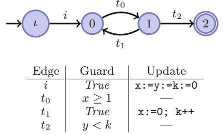
Fig. 2. Real-time program P_2
