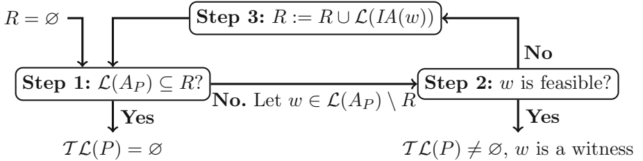
Fig. 3. Trace abstraction refinement semi-algorithm for real-time programs
