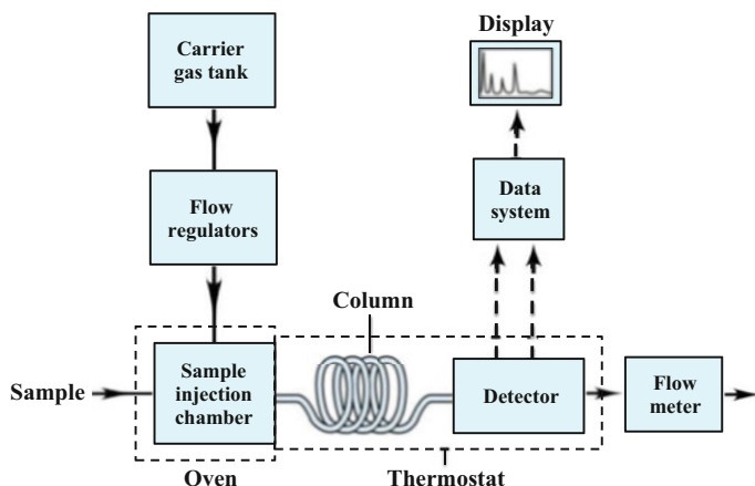
Fig. 13.1 Schematic diagram of gas chromatography (GC)
