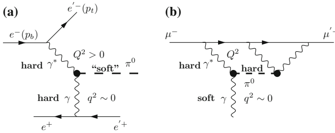
Fig. 5.57 a Measurement of the \pi^0 form factor \mathcal{F}_{\pi^0\gamma^*\gamma}(m_\pi^2, -Q^2, 0) at high space-like Q^2 , b needed at external vertex is \mathcal{F}_{\pi^0\gamma^*\gamma}(-Q^2, -Q^2, 0)
