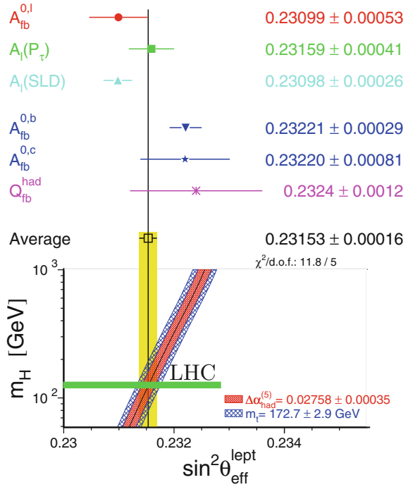
Fig. 4.16 Plot of the LEP Electroweak Working Group: S. Schael et al. 2005 [135], superimposed with the LHC result. [Resource CERN]
