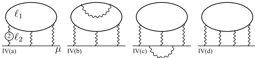
Fig. 4.9 Some typical diagrams of subgroups IVa (54 diagrams), IVb (60 diagrams), IVc (48 diagrams) and IVd (18 diagrams). The lepton lines as in Fig. 4.6
