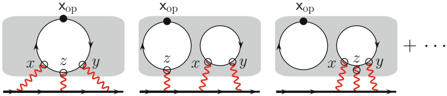
Fig. 5.85 Setup for the stochastic QED approach to HLbL. Connected and leading disconnected diagrams. Closed loops are quark loops decorated in all possible ways by non-perturbative gluon exchange. Photon vertices are to be permuted in all possible ways. One needs to make sure that the loops are connected by gluons, while vacuum blobs need to be subtracted, such that the diagrams are 1-particle irreducible. See also Fig. 5.86
