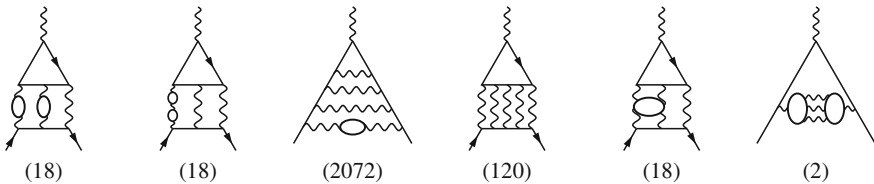
Fig. 4.11 Some typical tenth order contributions to a_e including fermion loops. In brackets the number of diagrams of the given type
