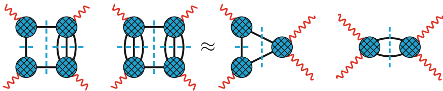
Fig. 5.71 Partial-wave approximation of multi-particle intermediate states by leading two-particle cut contributions
