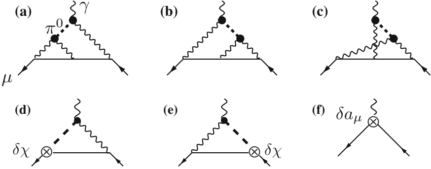
Fig. 5.63 Diagrams contributing to a_{\mu}^{\text{LbL};\pi^0} in EFT. \otimes denotes a renormalization counter term insertion. Counter terms \delta\chi are needed to render the triangular subgraphs of (a) and (b) finite, \delta a_{\mu} is needed to remove the remaining overall two-loop divergence
