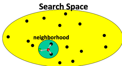
Fig. 10.2: Single-walk parallelism
