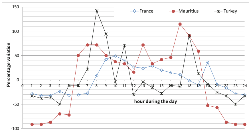
Fig. 7 Percentage variation of the hourly flow rate with respect to the average daily flow rate in three hospitals [1, 55, 57]
