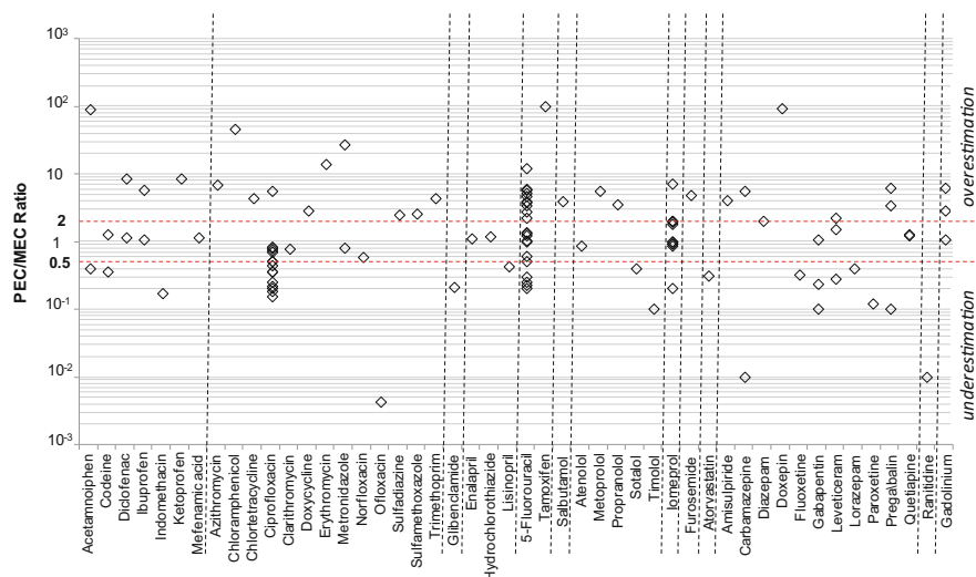
Fig. 8 Ratio between PEC and MEC for a selection of compounds grouped according to their therapeutic class. Horizontal dotted lines (corresponding to PEC/MEC equal to 0.5 and 2) define overestimation and underestimation regions as well as good accordance according to the criteria suggested by Ort et al. [58]. Data from: [15, 20, 21, 28, 33, 34]
