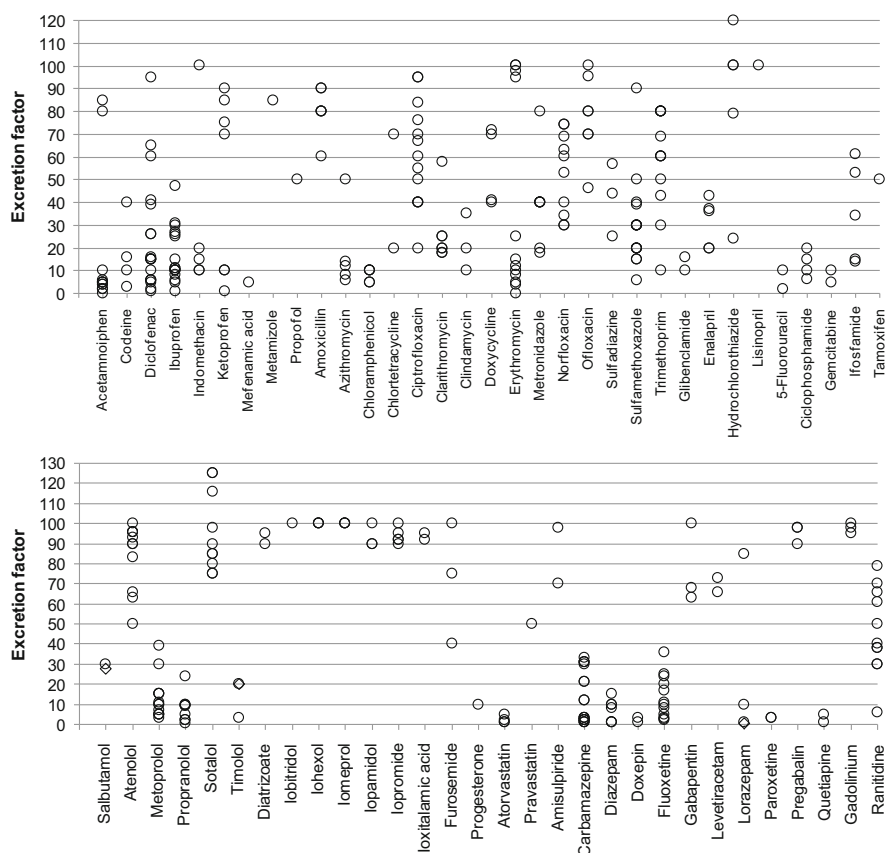
Fig. 3 Range of variability of the excretion factors reported in literature for the selected compounds. Data from: [2, 7, 10, 15, 17, 18, 22, 28, 31–33, 41–52; http://www.bioagrimix.com/hacpp/html/tetracyclines.htm ; http://www.ncbi.nlm.nih.gov/pmc/articles/PMC90863 ; http://www.ncbi.nlm.nih.gov/pubmed/3557734 ; http://www.medsafe.govt.nz/profs/datasheet/Daoniltab.pdf ; http://www.medsafe.govt.nz/profs/datasheet/b/Buventolinhalpwd.htm ; http://dmd.aspetjournals.org/content/3/5/361 ; http://www.ncbi.nlm.nih.gov/pmc/articles/PMC1428960/pdf/brjclinpharm00307-0061.pdf ; www.torino.medica.it ]
