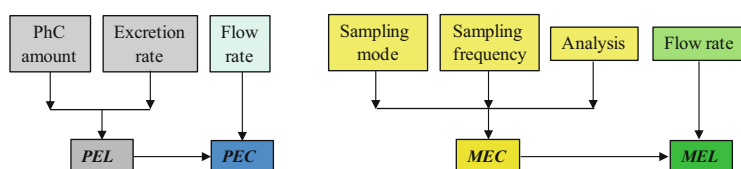
Fig. 1 Main parameters defining predicted and measured concentrations and loads of PhCs
