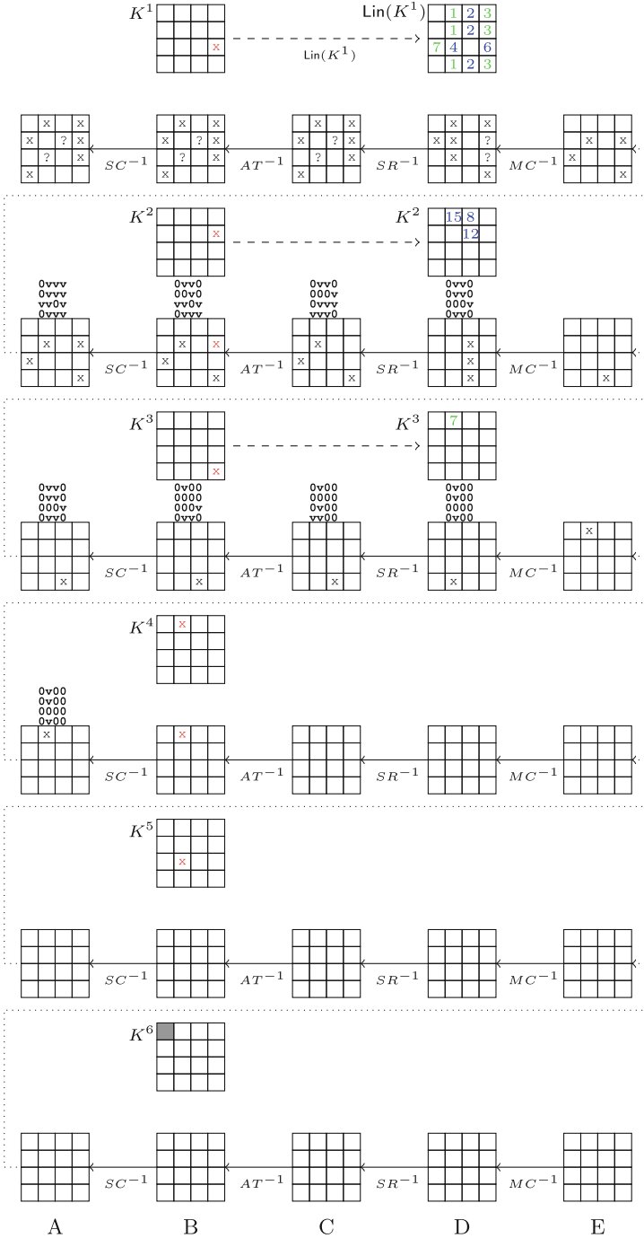
Fig. 4. Trail for the six forward rounds (the values of active nibbles in red are functions of \delta_1, \delta_2 , the dark gray cell visualises the tweakey cancellation). (Color figure online)
