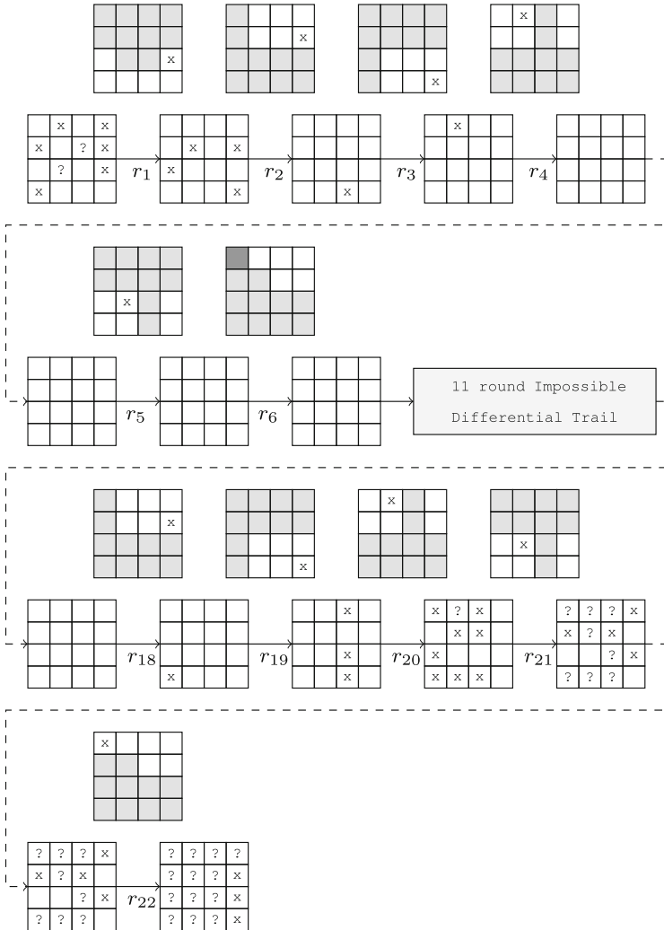
Fig. 9. Related-key impossible differential attack on 22 round SKINNY 64/128 (grey cells are the key, white cells are the tweak, the dark gray cell visualises the cancelation of the tweakkeys)
