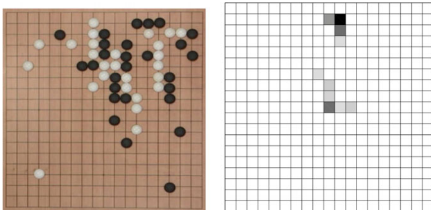
Fig. 10.13 Density graph ( right ) of a move probability p_\sigma(a|s) for the player with white stones in the board state shown on the left . For each white square, p_\sigma(a|s) = 0 . The darker the square, the higher the value for a move by white onto the corresponding grid point
