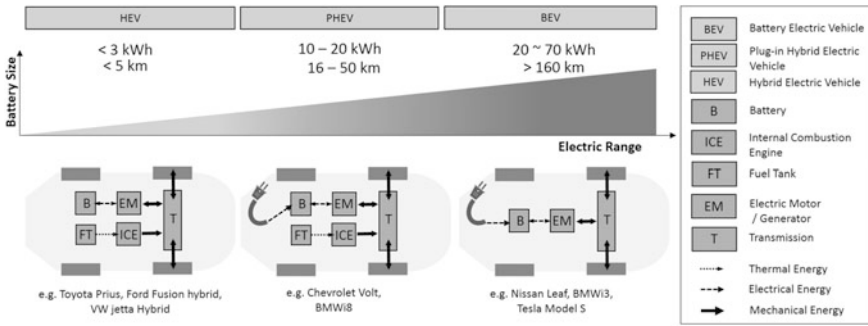
Fig. 27.1 Technical characteristics of electric vehicles
