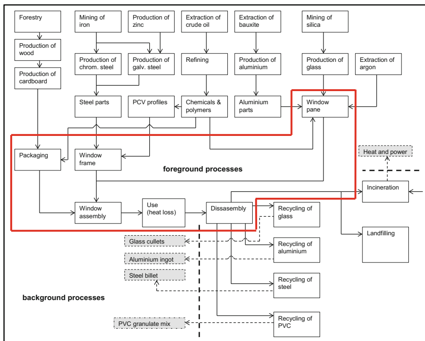
Fig. 39.6 Product system of the polyvinyl chloride window (PVC). Red line indicates foreground processes. Grey boxes indicate avoided processes
