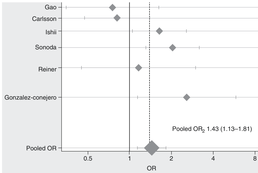
Fig. 3.2 This shows the odds ratio for the Met/Thr variant versus the Thr/Thr variant in glycoprotein GP1b \alpha and ischemic stroke. In this case, significant heterogeneity was present ( I^2 = 58\% , p value = 0.04) (Reprinted with permission from Maguire et al. [111])
