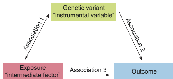
Fig. 3.3 Mendelian randomization (Adapted from Thanassoulis et al. [66])
