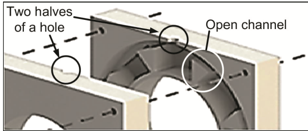
Fig. 3. Prototype model: channels for LN 2 cooling.
