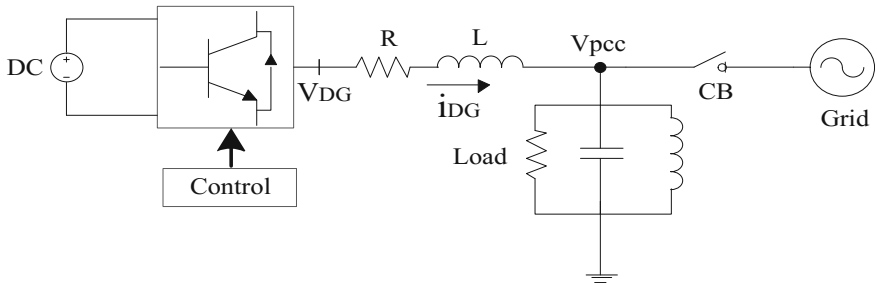
Fig. 1. DG with the local load connected to the grid.
