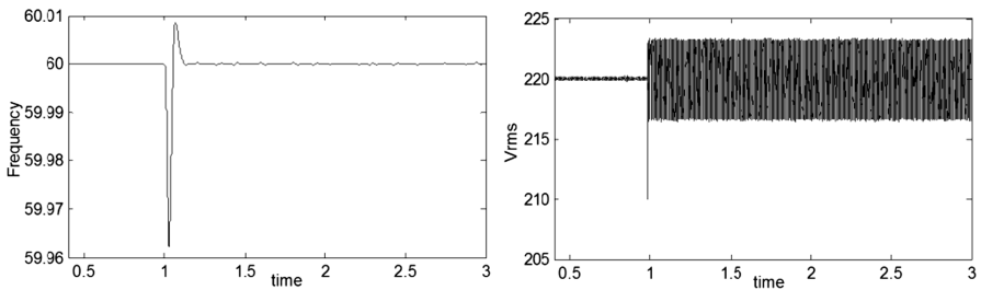
Fig. 7. Voltage and frequency of PCC with temporary reactive injection for low-quality load in Case 3.
