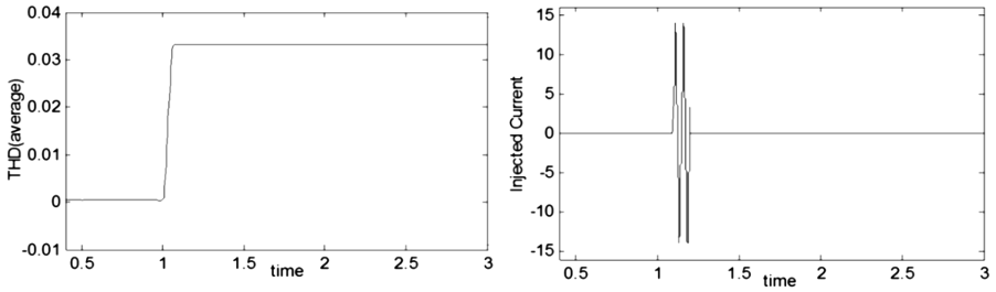
Fig. 6. The average of THD of the voltage at PCC and injected reactive current in Case 3.
