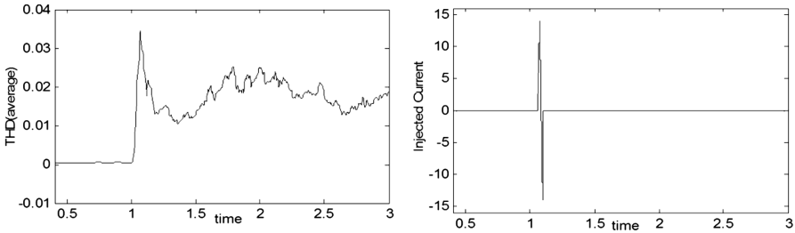
Fig. 4. The average of THD of the voltage at PCC and injected reactive current in Case 2.
