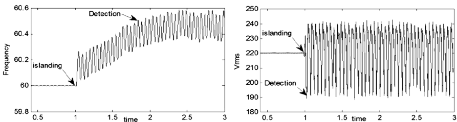
Fig. 3. Voltage and frequency of PCC with permanent reactive injection for low-quality load
