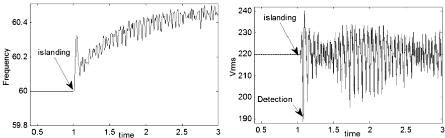
Fig. 5. Voltage and frequency of PCC with temporary reactive injection for low-quality load in Case 2.
