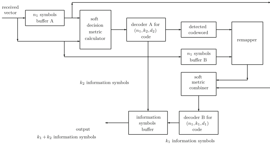
Fig. 16.3 Decoder for the concatenated code with the codeword format shown in Fig. 16.1
