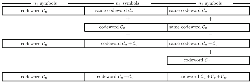
Fig. 16.5 Format of transmitted codeword consisting of two levels of concatenation and three shorter codewords
