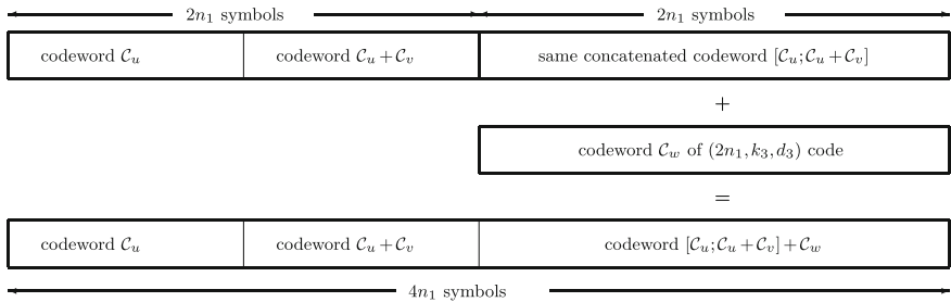
Fig. 16.6 Format of transmitted codeword after two stages of concatenation
