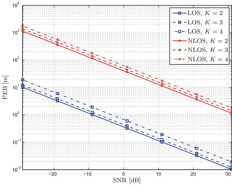
Fig. 9.20 Performances of the PEB for the LOS in presence of clusters and NLOS conditions with different number of clusters \mathbf{s}_k \text{ [m]} = [1.5, 1 + (k - 1) \times 0.1]^T for k = 2, \dots, 4 , \mathbf{q} \text{ [m]} = [0, 0]^T , and \mathbf{p} \text{ [m]} = [0, 4]^T
