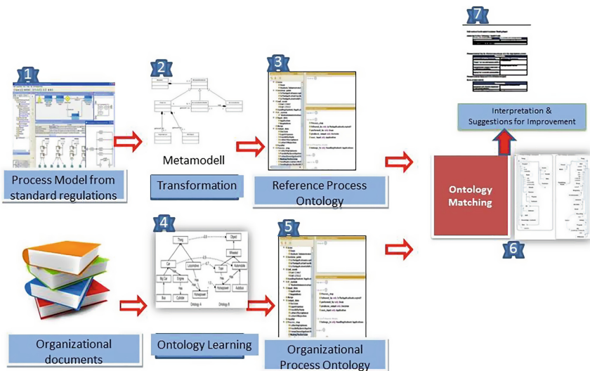
Fig. 2. Processes of the semantic audit application
