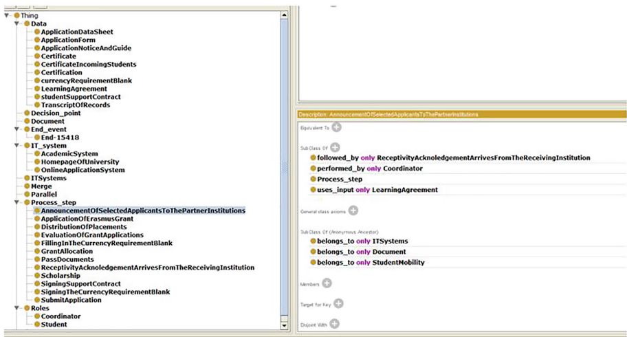
Fig. 1. Reference process ontology
