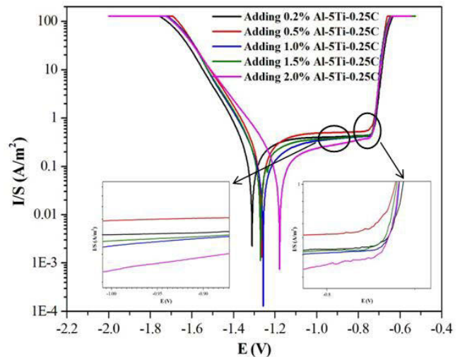
Fig. 4 Polarization curves and its partial enlarged view of 6063 alloy samples inoculated by Al-5Ti-0.3C master alloy.
