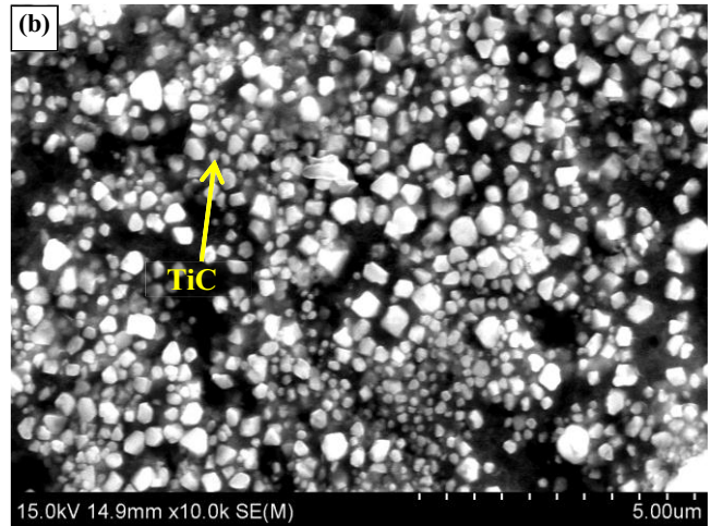
Fig. 1 Microstructures of (a, b) Al-5Ti-0.3C master alloy.
