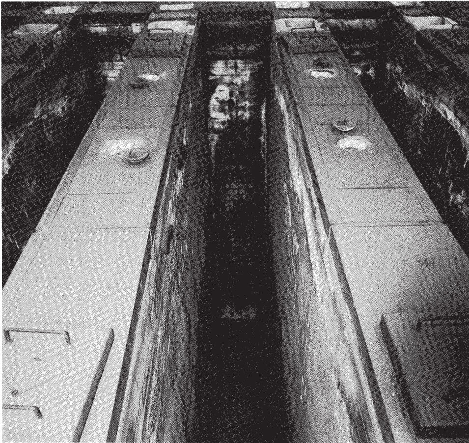
figure 8: Flue according to the "state of the art 1985" after 50 fire cycles
