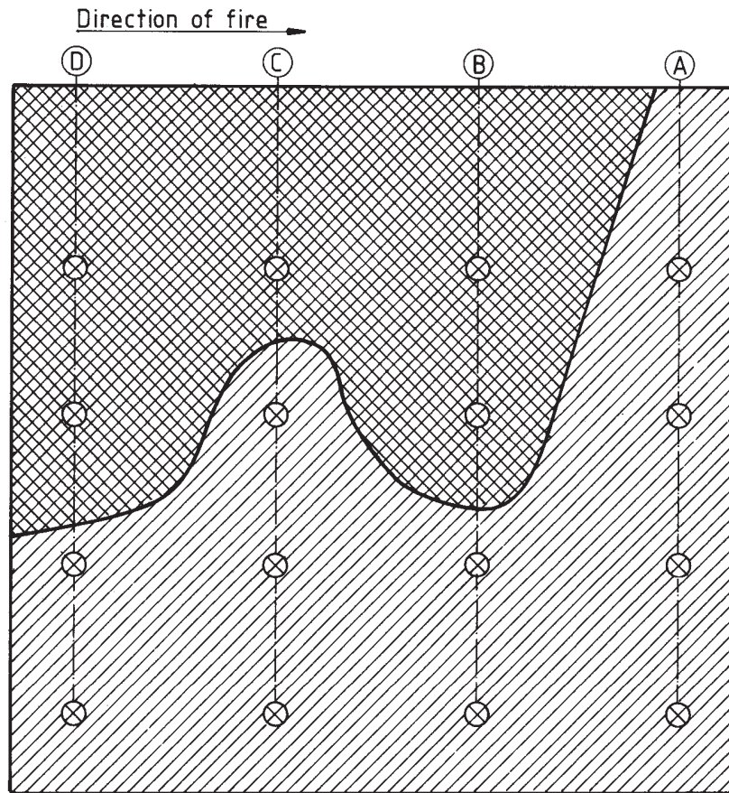
figure 4: Temperature distribution according to the "State of the art 1985" (same scale as figure 3)
