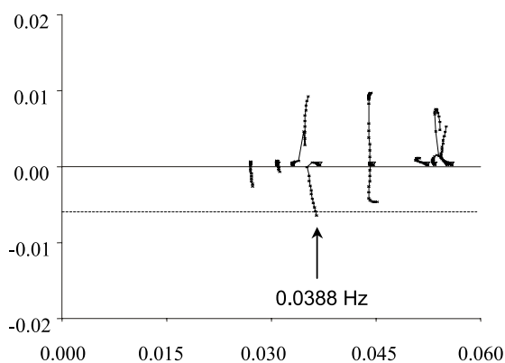
Figure 14 : Stability diagram after the "dirty" AC
