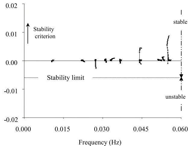
Figure 3: Stability diagram for a healthy pot at ISAL, operating at 147 kA
