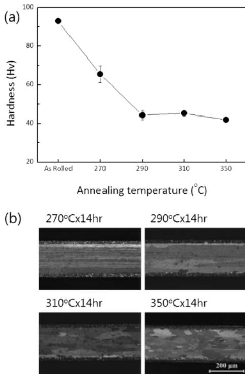
Figure 2. (a) Vickers hardness and (b) optical micrographs with respect to the annealing temperature.
