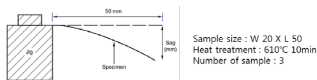
Figure 1. Schematics of sag test [6]
