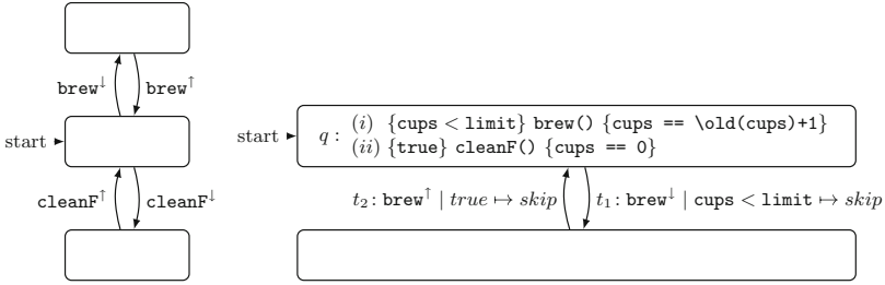
Fig. 3. (left) The control-flow graph of the system under scrutiny; and (right) an optimised 4 specification of brewing of coffee leaving out unnecessary checks
