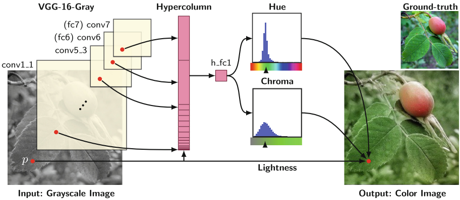
Fig. 2. System overview. We process a grayscale image through a deep convolutional architecture (VGG) [36] and take spatially localized multilayer slices (hypercolumns) [14,25,27], as per-pixel descriptors. We train our system end-to-end for the task of predicting hue and chroma distributions for each pixel p given its hypercolumn descriptor. These predicted distributions determine color assignment at test time. (Color figure online)
