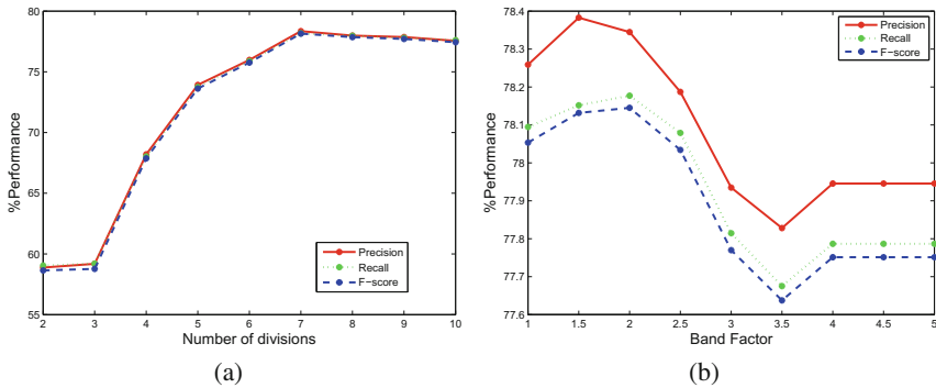
Fig. 3. The performances with the increase of (a) the number of divisions and (b) the value of band factor on the Chalearn Gusture dataset
