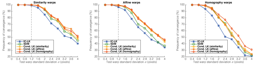
Fig. 6. Frequency of convergence comparison between IC-LK, SDM, and Conditional LK trained with 100 examples per layer and tested with swapped warp functions. The parentheses indicate the type of warp function trained with.
