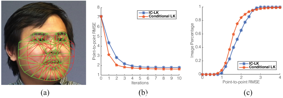
Fig. 11. (a) An example of facial model fitting. The red shape indicates the initialization, and the green shape is the final fitting result. (b) Convergence rate comparison between IC-LK and Conditional LK. (c) Comparison of fitting accuracy. (Color figure online)
