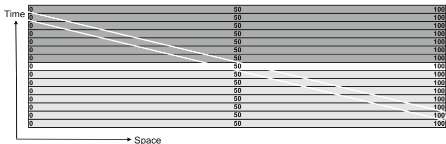
Fig. 11.5 The worldtube of the meter stick with different colors
