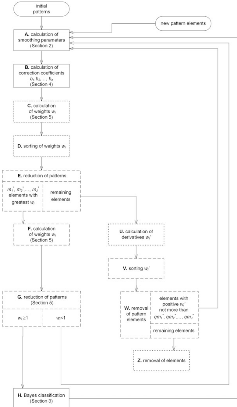
Fig. 1 Classification metaheuristic
