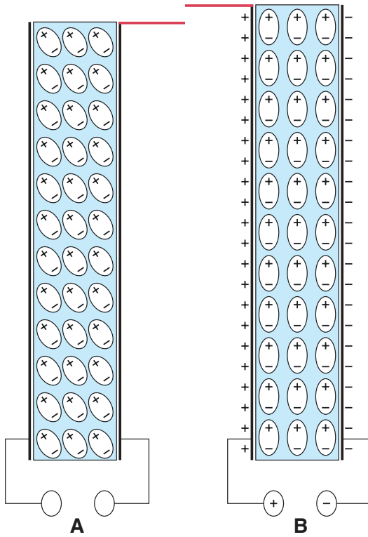
Fig. 5.5 The piezoelectric effect. When a piezoelectric crystal is placed in an electromagnetic field, the molecular dipoles align causing a physical change in the shape of the crystal. An alternating electric current will cause distortions in the shape of the crystal, thereby converting electrical energy into mechanical energy and vice versa. From R. Sofferman and A. Ahuja, Ultrasound of the Thyroid and Parathyroid Glands . Springer 2012
