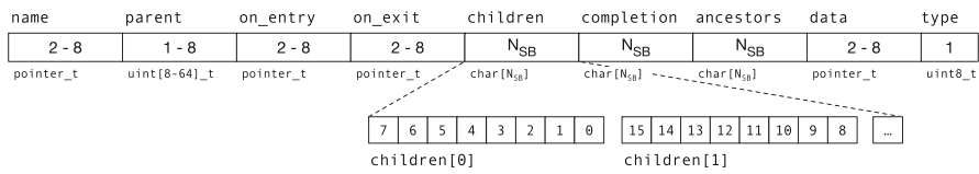
Fig. 10.2 The memory representation of a single state structure depends on the target platform’s bit-width, the total number of states and any eventual padding
