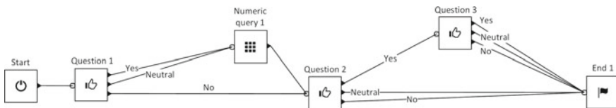
Figure 1 Example for a visual program
