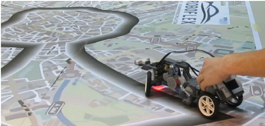
Figure 4 Autonomously driving Lego Mindstorms NXT robot in ROBOFLEX
