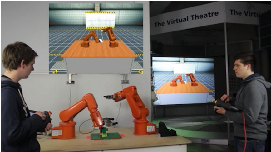
Figure 4 Manual control of the robots and visual representation in the Virtual Theatre
