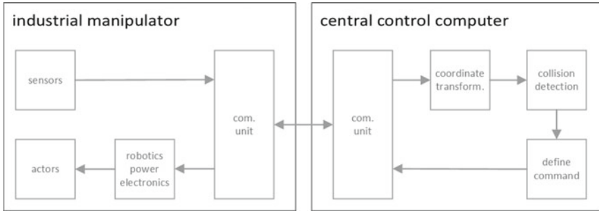
Figure 2 Signal flow
