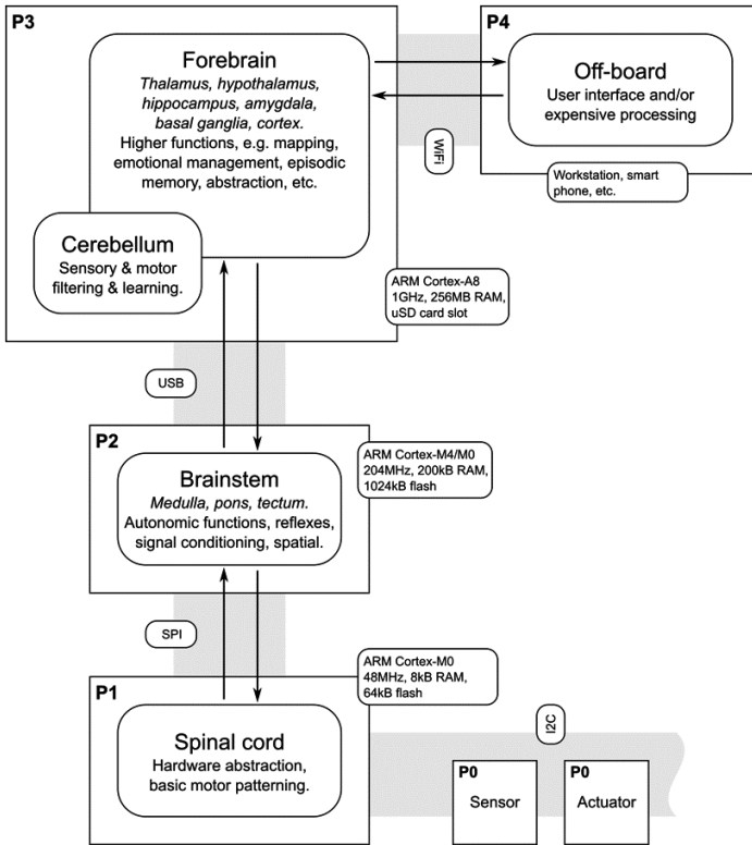
Fig. 4. The biomimetic MIRO control architecture is implemented across three on-board processors, P1-3, each loosely associated with a broad region of the mammalian brain. The design physically displays dissociation, since P2 (and, to a more limited extent, P1) is able to control the robot independently of higher processing layers. “P4” denotes off-board processing, and “P0” non-reprogrammable peripheral-specific processors.
