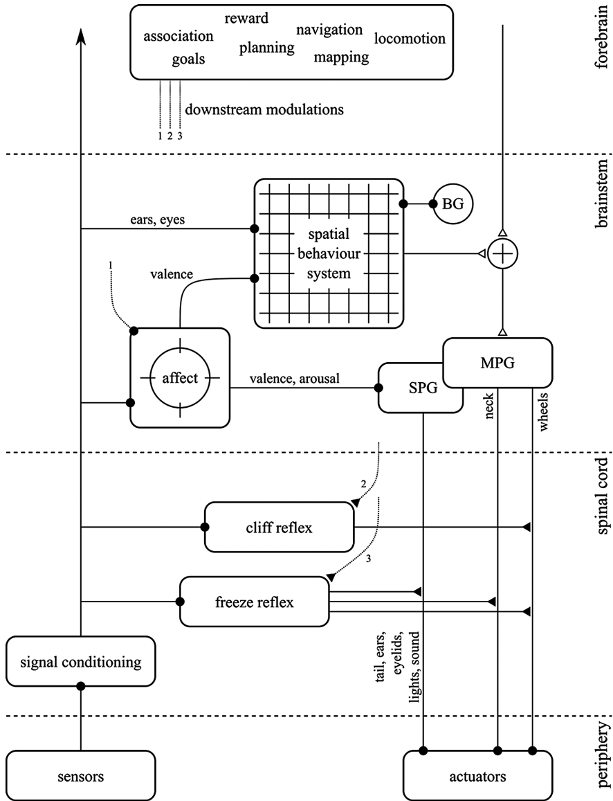
Fig. 3. Control architecture of MIRO loosely mapped onto brain regions (spinal cord, brainstem, forebrain). Signal pathways are excitatory (open triangles), inhibitory (closed triangles), or complex (closed circles). See text for description of components.
