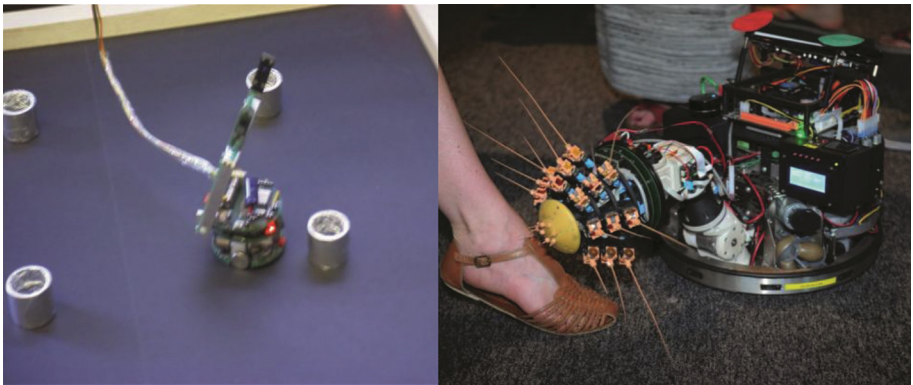
Fig. 1. Neurobotic models of control architectures. Left: [4] embedded a model of the vertebrate basal ganglia in a table-top robot and showed its ability to control action selection and behavioural sequencing for a simulated foraging task. Right: Shrewbot [5] is one of series of whiskered robots developed to explore the effectiveness of brain-based control architectures in generating life-like behaviour.
