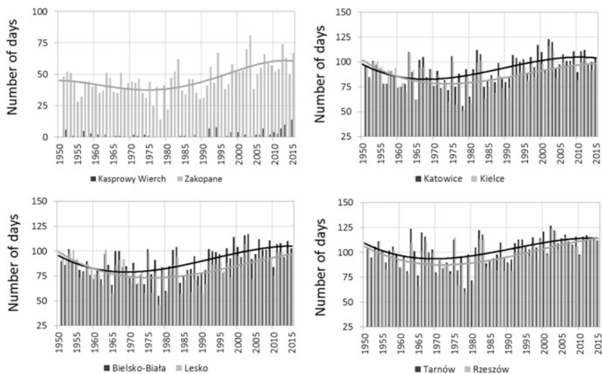
Fig. 6 Annual number of summer days ( T_{\text{mean}} \geq 15 \text{ }^\circ\text{C} ) at selected stations in the Upper Vistula Basin in the 1951–2015 period ( bars —observed number of days, lines —fitted 3rd [Zakopane] and 4th order polynomial)
