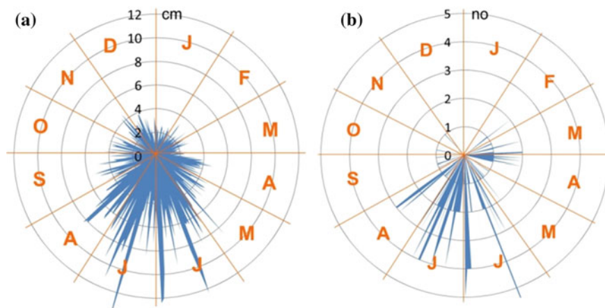
Fig. 4 Hydrometeorological situation at the northern foothills of the Tatra Mountains: a Average precipitation (cm) from 19 meteorological stations (28 years: 1954–1982); b Number of water flow larger than 1.5 times than averages as measured at Nowy Targ water gauge for the period 1898–1983 (Ballesteros-Cánovas et al. 2015a). After Ballesteros-Cánovas et al. (2015a), published by permission of Elsevier
