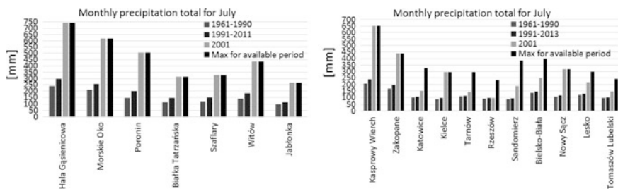
Fig. 18 Comparison between mean monthly precipitation total for July in the period 1961–1990 with the mean value from period 1991–2011 ( left ) or 1991–2013 ( right ); the value for July during flood 2001 year and the maximum value for all research period
