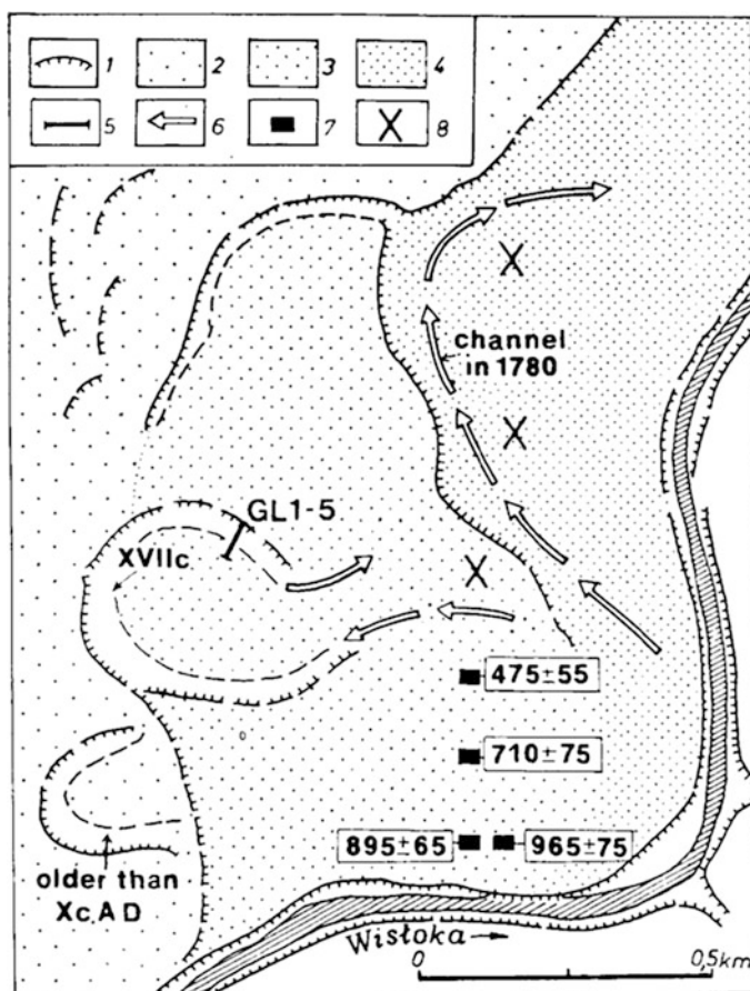
Fig. 10 Terrace levels and palaeochannels in the Wistoka River valley near Grabiny (after Starkel 2001). 1 Edges of terraces, 2 terrace level 8–9 m, 3 terrace level 7 m, 4 terrace level 4 m, 5 cross-section, 6 course of palaeochannel, 7 dated buried trees
