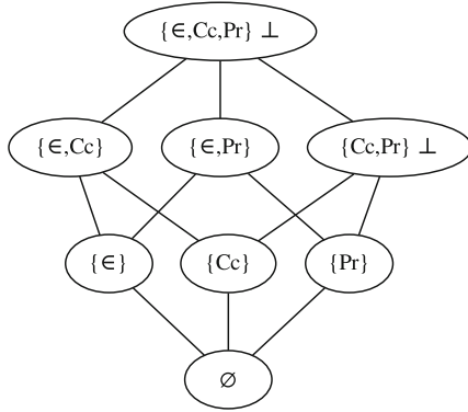
Fig. 2. The indiscernibility lattice for the graph in Fig. 1. For readability we abbreviate tbody:chemComp as Cc , tbody:prod as Pr , rdf:type as €, and owl:sameAs as \sim . Two of the indiscernibility relations cannot be chosen without resulting in an inconsistent state.
