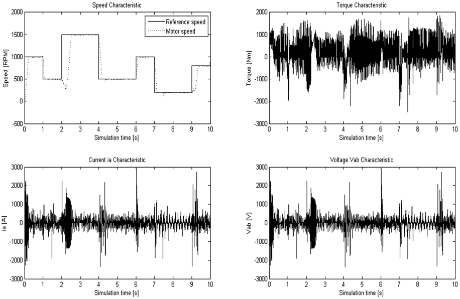
Fig. 6. Results for 100 Nm load.
