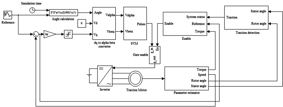
Fig. 1. Model of the proposed system
