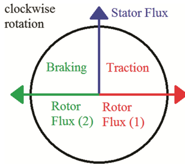
Fig. 3. Fluxes positioning and effect
