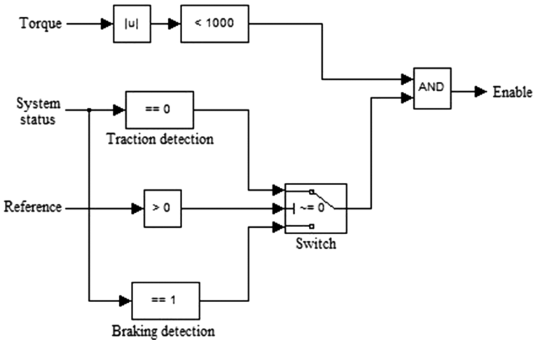
Fig. 2. Model of the “Gate Enable” block
