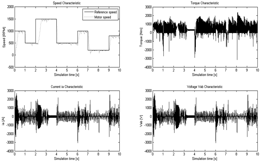
Fig. 7. Results for 300 Nm load.
