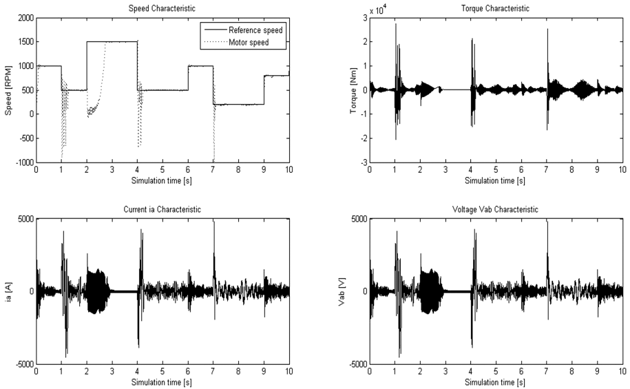
Fig. 8. Results for 100 Nm load, without using the filters described in subchapter 3.3.
