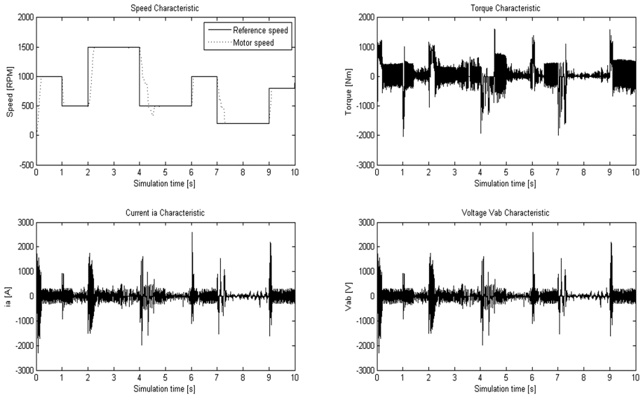
Fig. 5. Results for 10 Nm load.
