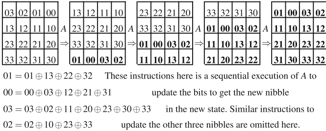
Fig. 3. MixColumnsSerial of LED operate on one column
