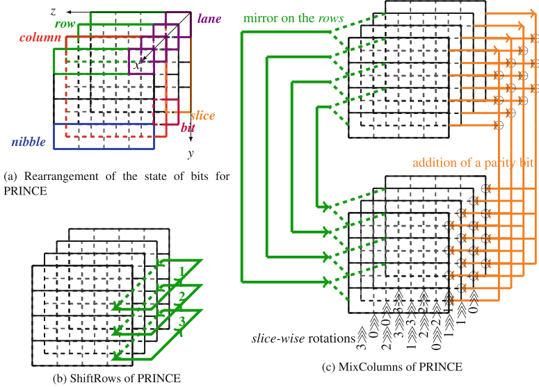
Fig. 2. Rearrangement of the state of bits, ShiftRows and MixColumns of PRINCE
