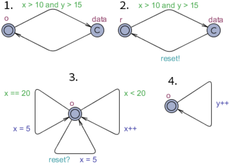
Fig. 5. Timed automata describing the security policy \{o(x[20; ?reset; 5] > 10 \ \&\& \ y > 15) : r[!reset]\}
