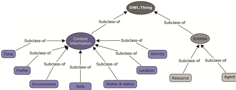
Fig. 1. Upper-level ontology.
