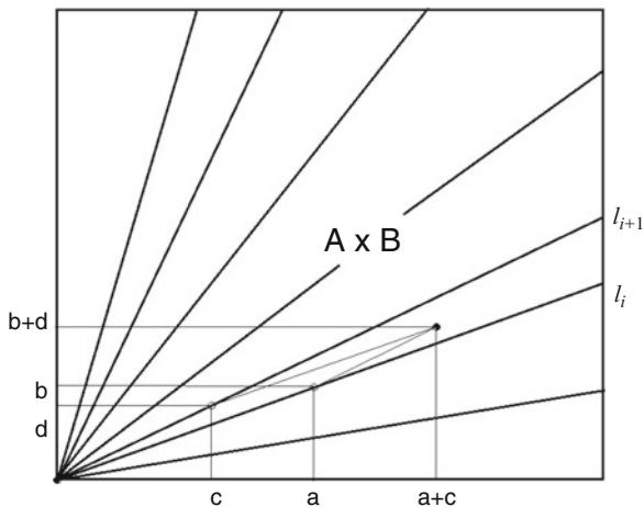
Fig. 1 The sum of (a, b) \in \ell_i and (c, d) \in \ell_{i+1} is a unique point of the Cartesian product (A + A) \times (B + B) .
