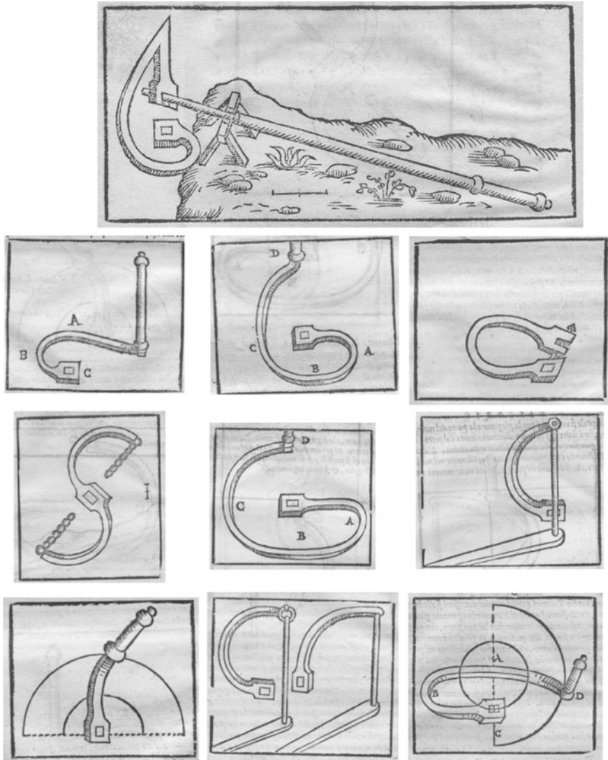
Fig. 17 An author of the same era, in order to improve the efficiency of the machine, was working on ... the shape of the crank (Ceredi 1567)
