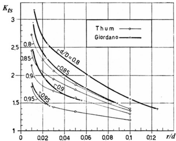
Fig. 6 Stress concentration factors K_{ts} = \tau_{max}/\tau_n for shouldered shafts (smaller diameter/larger diameter = d/D ) subjected to torsion vs the ratio r/d between the radius of the fillet and the diameter d of the smaller shaft (based on a figure taken from Giordano 1940c)
